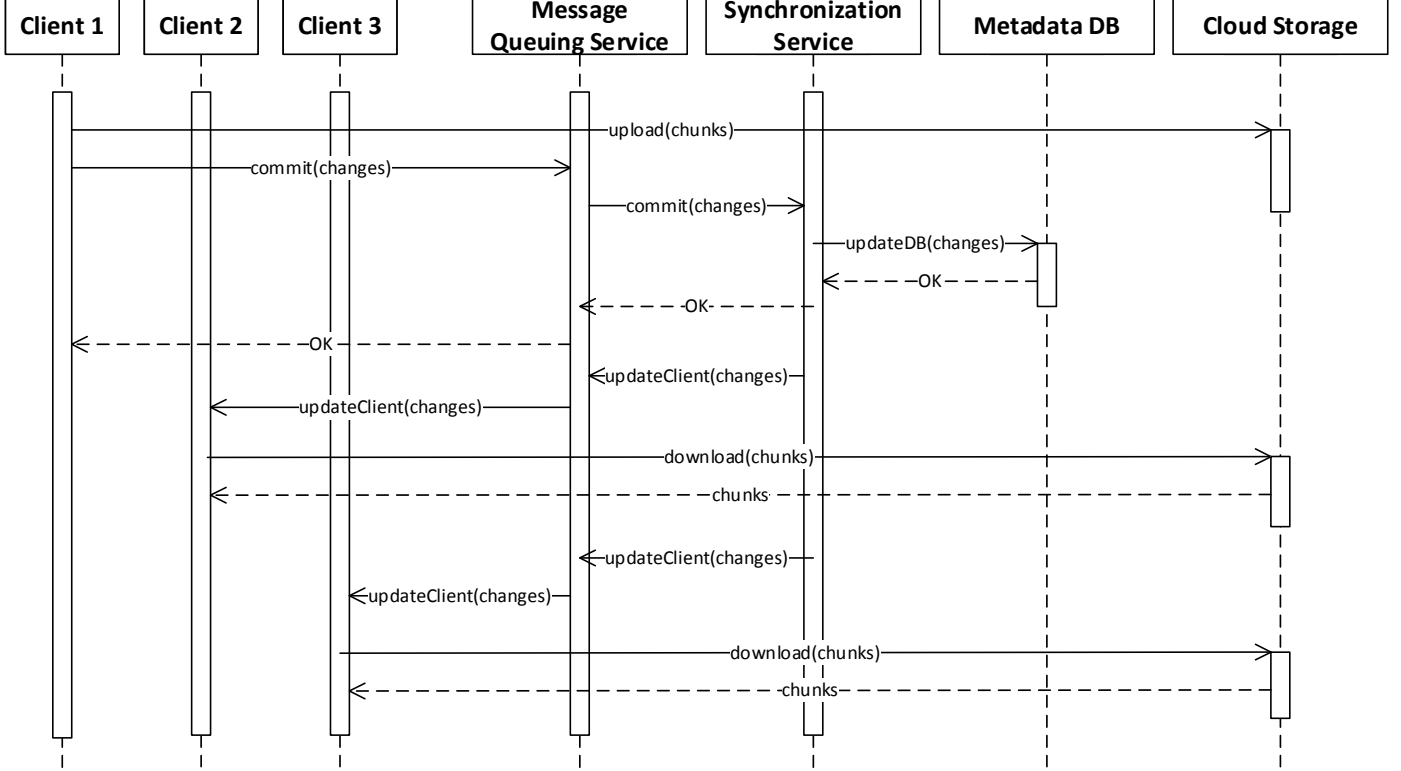
Figure 4. Sequence Diagram
