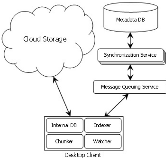
Figure 2. Logical Architecture
